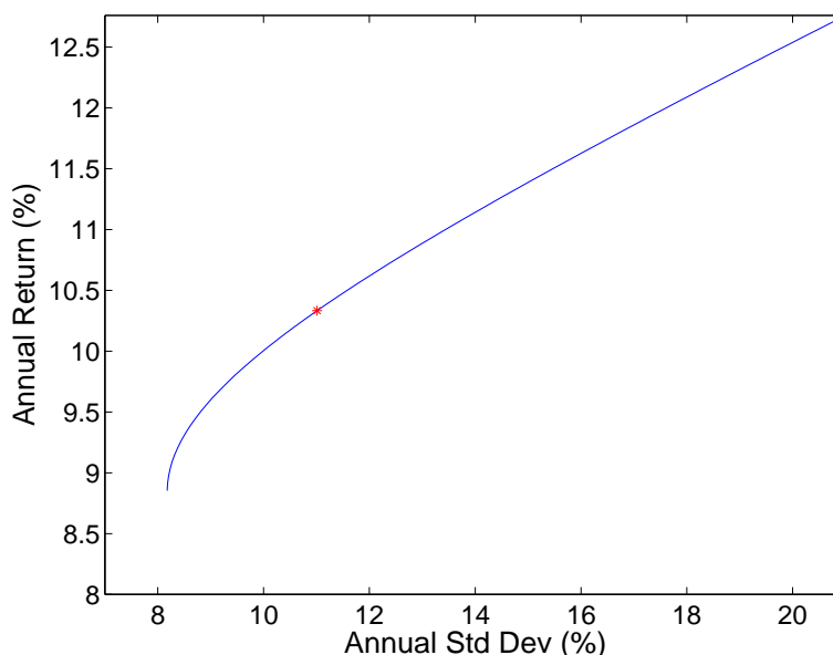
Fig. 2. Efficient frontier of two risky asset case with the optimal portfolio for quadratic utility ( \alpha = .33 ) labeled.
