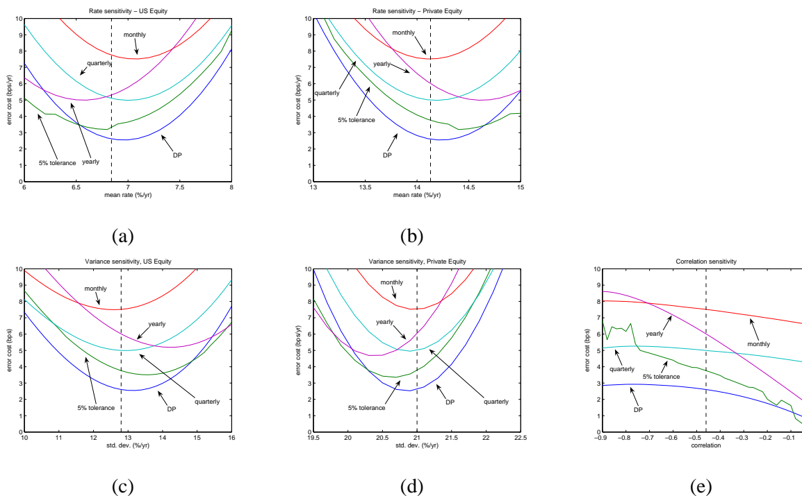
Fig. 4. Sensitivity analysis on mean, standard deviation, and correlation for two asset example. The vertical line indicates the rate used by the rebalancing strategies. (a) Sensitivity to mean rate for US Equity. (b) Sensitivity to mean rate for Private Equity. (c) Sensitivity to variance for US Equity. (d) Sensitivity to variance for Private Equity. (e) Sensitivity to correlation between US and Private Equity.
