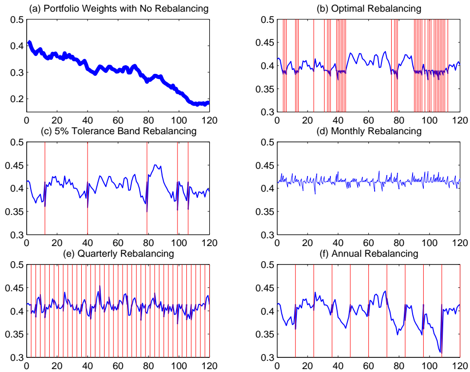
Fig. 3. Plots of US Equities weighting in the two asset example using different rebalancing models. The vertical lines indicate months where rebalancing was done (for monthly rebalancing, this is omitted since trading occurs in every month).
