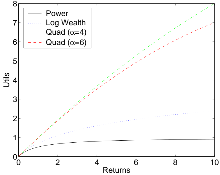
Fig. 1. Plots of the quadratic utility (for two different \alpha 's), log wealth utility, and power utility as a function of returns.
